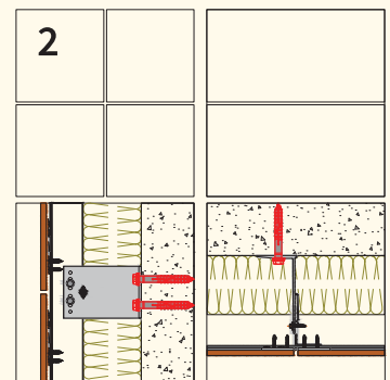
2. 'Z - Profile' system
